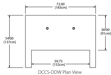
DCCS-DDW Plan View
