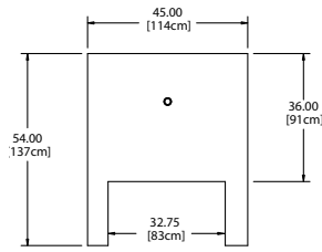
DCCS-SDW Plan View
