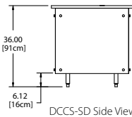
DCCS-SD Side View
