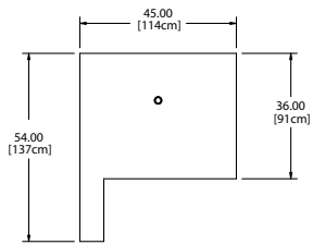
DCCS-SDWL Plan View
