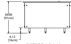
DCCS-DDW Side View
