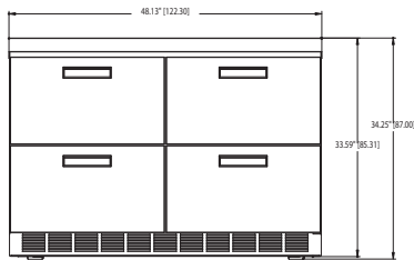
UCD4448N Elevation View
