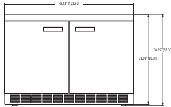
UC4448N Elevation View
