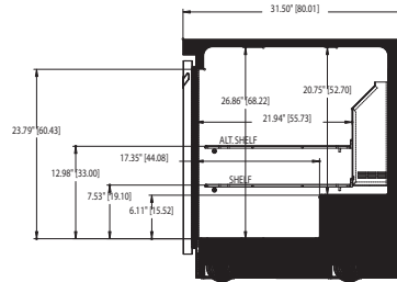
UC4448N Right Side View
