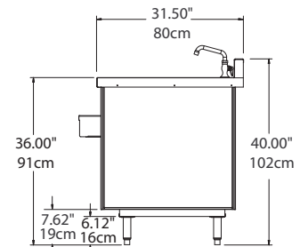
End View All Models
