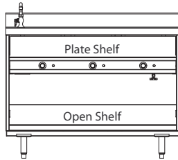
Elevation View F14EI348
