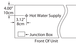
Mechanical Data Plan View All Models
