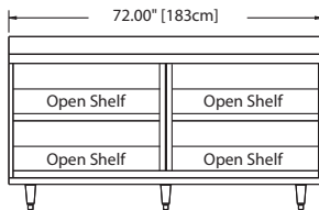
Elevation View F16OS72
