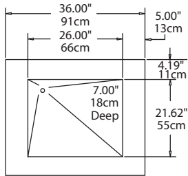
Plan View KCSC-36-BP
