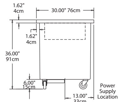
Typical End View All KCSC-BP Models
