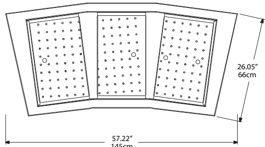
N8059-R Plan View
