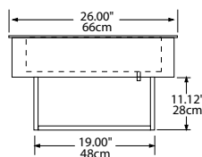
Right End View, N8118BP
