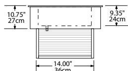
Elevation View, N8118BP
