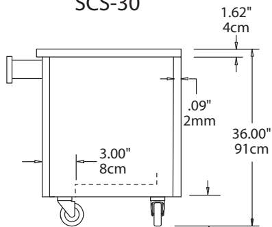
End View SCS-30
