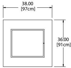
DC-FT2P Plan View
